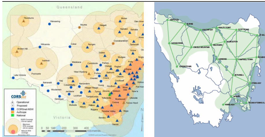
Figure A.5 CORS networks in New South Wales and Tasmania
