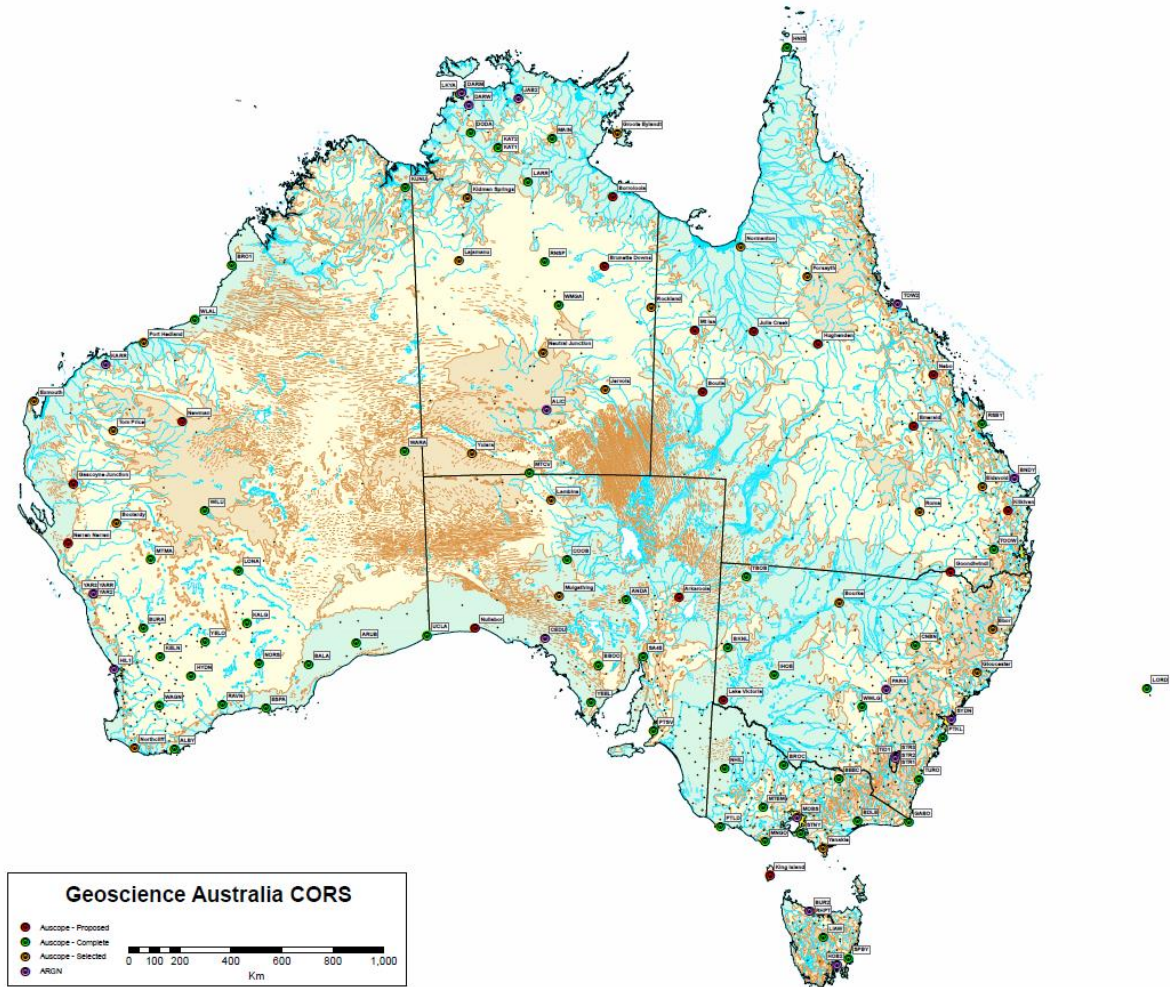
Figure A.4 The AuScope CORS network
