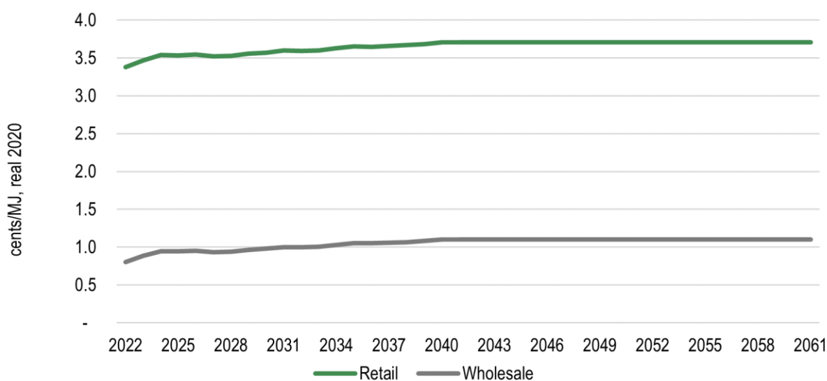
Figure 2.14 Comparison of gas prices at wholesale and retail prices, cents per MJ
